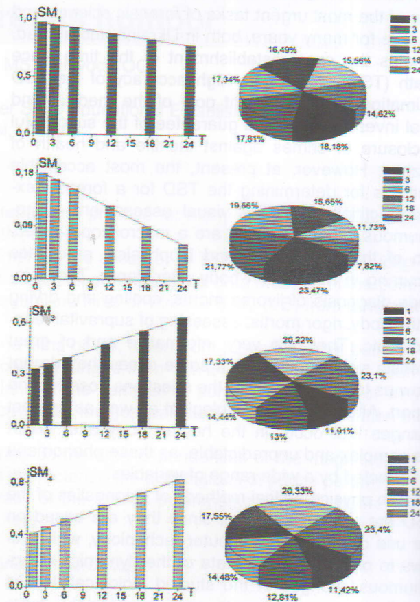
Fig. 2 Time charts of the change in the magnitude of the statistical moments of the 1st-4th order (SM i ), that characterize the distributions of the PP of the Stokes vector of the microscopic images of VB layers of the deceased with different TSD (T, h.)
