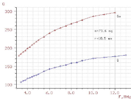
Fig. 2. Dependences of the quality factor Q of the oscillating solenoid circuit on the resonant frequency f in the presence ( Q ) and absence ( Q_0 ) of an aluminium disc
